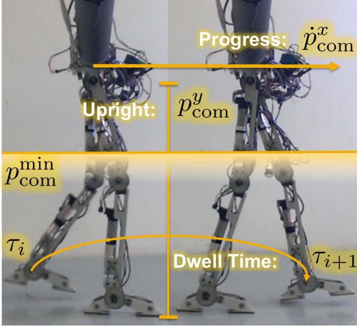
(a) Graphical illustration of the definition of walking.
