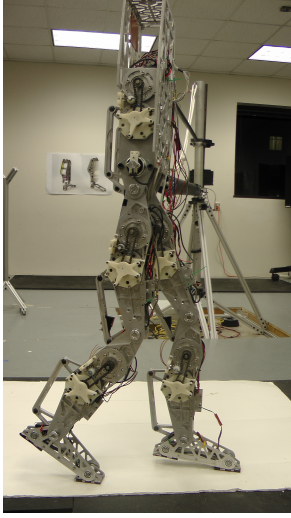
(a) Sideview of bipedal robot AMBER 3.
