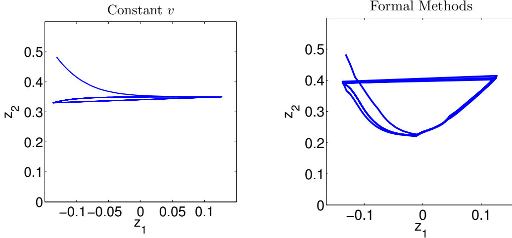
(c) Phase portrait for the zero dynamics coordinates (z_1, z_2) over four steps. In both cases, the controller induces stable limit cycles in these coordinates
