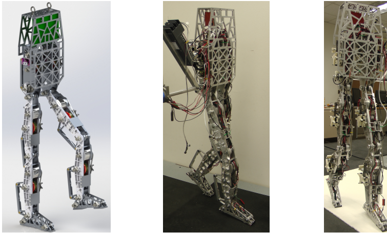
Figure 2: Bipedal walking robot AMBER 3.
