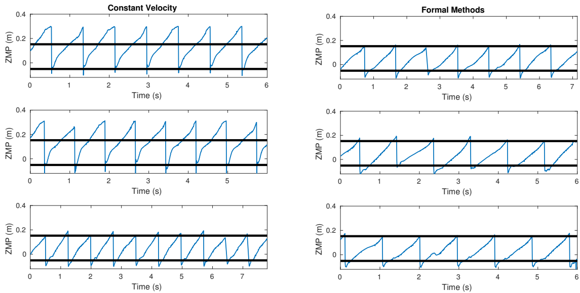
Figure 11: The location of the zero moment point relative to the point on the ground directly below the stance ankle. The black lines represent the boundaries of the foot; when the blue line indicating the instantaneous position of the ZMP leaves the region bounded by the black lines, a violation of the ZMP constraint occurs, allowing the foot to roll about its extremities. The portion of time the ZMP remains within the foot is 0.4975, 0.4835 and 0.7902 for the constant v trials and 0.8352, 0.7652, and 0.7942 for the formal methods controller.
