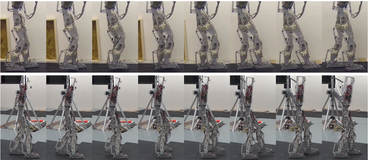
Figure 8: Tiles of the walking gait generated by the formal methods controller (video at [1].) The images in the top row are from the point of view of the boom. The images in the bottom row were taken from outside the radius of the boom.
