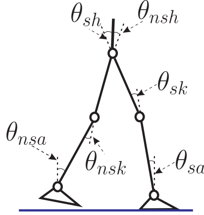
(b) Joint angles.
